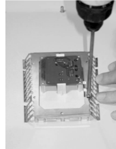
9. Align screw openings of the stainless steel bracket in the platform holes with screws. Screw six (6) screws in place.
