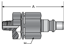
HP006-2-NMB HP006-2-NMC HP006-2-NMD
